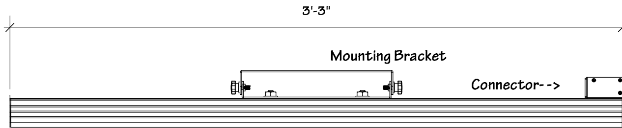
Front view (Light panel point downward)
